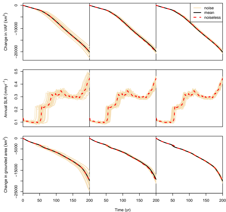
Figure 6. Change in ice volume above floatation (VAF), annual sea level rise (SLR) and change in grounded area for the PIG basin (Fig. 2a, d). The three columns are for experiments with lower- (left), medium- (middle) and higher- (right) frequency noise on the bedrock. Higher-frequency noise leads to less variation than low-frequency noise, while the mean over all of the experiments with noise added is close to the noiseless experiment. Much of the variation is associated with the onset of rapid retreat at around 50 years, evident in the plot of annual SLR.
