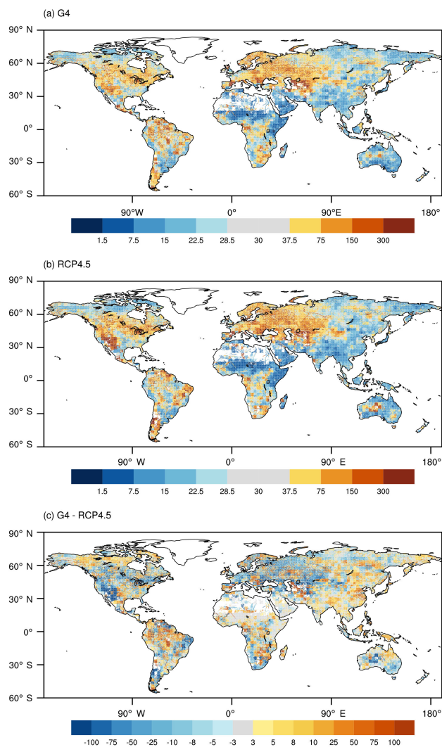
Figure 5. Multi-model ensemble median of return periods for discharge that correspond to a 30-year return period level in the historical simulation (1960–1999) under (a) G4, (b) RCP4.5, and (c) the difference of G4 and RCP4.5. Grid cells in extremely dry regions in the historical simulation, i.e., Q_m < 0.01 \text{ mm day}^{-1} , are masked out.
