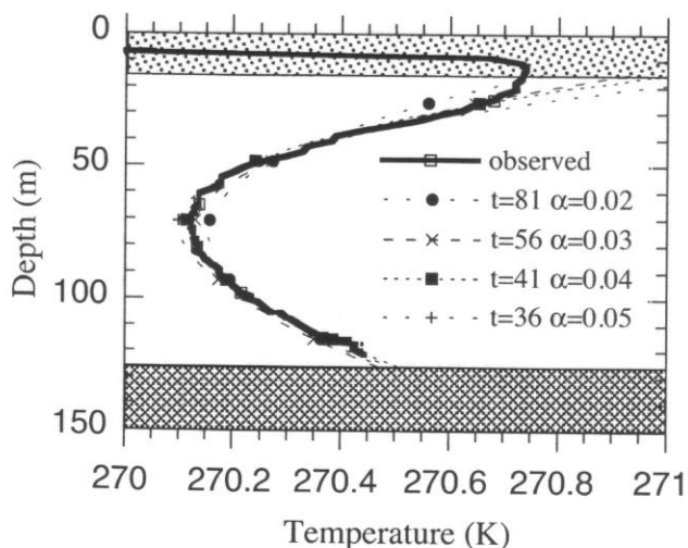
Fig. 4. Temperature profiles for different values of \alpha (\text{K a}^{-1}) , showing the snapshots in time which resulted in the best match between observation and calculation for a particular value of \alpha . Parameters: H = 126.5 , G = 25 \text{ mW m}^{-2} , w_s = -0.38 \text{ m a}^{-1} , linear profile.
