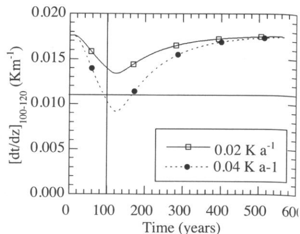
Fig. 5. The evolution of the temperature gradient near the bottom of the core in the case of an increase of 0.02 and 0.04 \text{ K a}^{-1} over a period of a 100 years (indicated by the vertical line). The horizontal line indicates the observed gradient in this section. Parameters: H = 126.5 \text{ m} , G = 37.5 \text{ mW m}^{-2} , w_s = -0.38 \text{ m a}^{-1} , linear profile.
