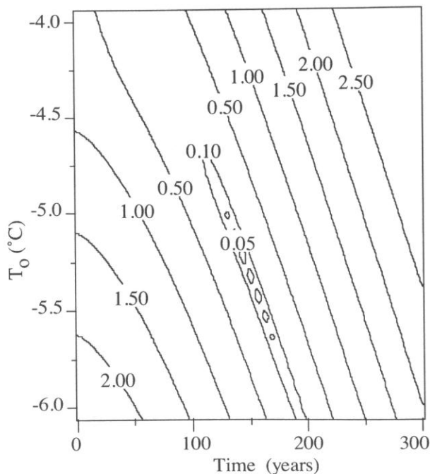
Fig. 7. Typical example of the rms error between the observations and the calculations for the variables T_0 and t . The other parameters are constant: H = 126.5 \text{ m} , G = 37.5 \text{ mW m}^{-2} , \alpha = 0.025 \text{ K a}^{-1} , w_s = -0.38 \text{ m a}^{-1} and a quadratic profile.
