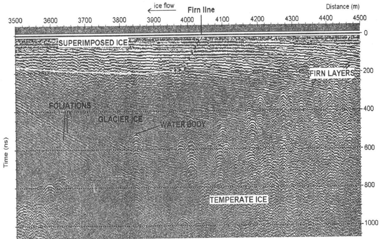
Fig. 2. 50 MHz radar profile from Werenskiöldbreen. Dipping foliations are seen clearly in the cold ice, and a strong hyperbolic diffraction indicating a likely water body. Much radar clutter is seen in the temperate ice underneath the cold-ice layer. The region of superimposed ice, estimated by the presence of weaker sub-parallel layering and sporadic hyperbolic diffractions down-glacier of the firn line, is delimited by the white line and, where it is hard to determine, by the dashed line. The number of firn layers indicates that the oldest firn is 10–15 years old.
