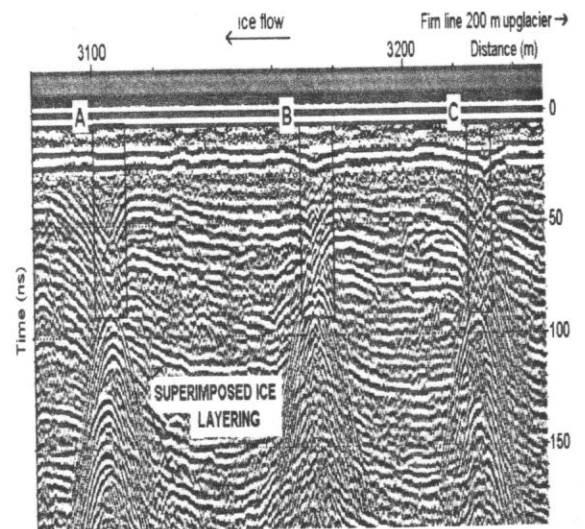
Fig. 6. Hyperbolic reflections (in boxes A, B, C) at 50–100 ns (5–10 m depth) \sim 200 m down-glacier of the firn line in 200 MHz data of Hansbreen, possibly indicating superimposed ice (cf. Figs 2–4). The down-dipping layers in the boxes could be due to enhanced water content in the ice, and the hyperbolic scattering indicates water contents of 1.2%, 3.3% and 3.6% for boxes A, B and C, respectively.
