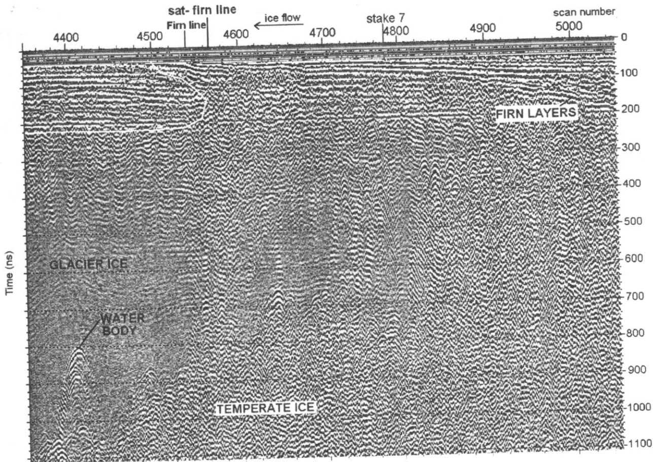
Fig. 4. The firn-ice transition in 50 MHz GPR data of Kongsvegen. The firn line from the GPR data and the satellite image (labelled as "sat-firn line"; see Fig. 5) is marked, along with the location of stake 7. The layering in the firn area is easily seen. We interpret the hyperbolic diffractions on top of warm ice and just before the line as water bodies. Superimposed ice marked by sporadic reflections around 200 ns and variable-strength sub-parallel reflections are delimited by the white line.
