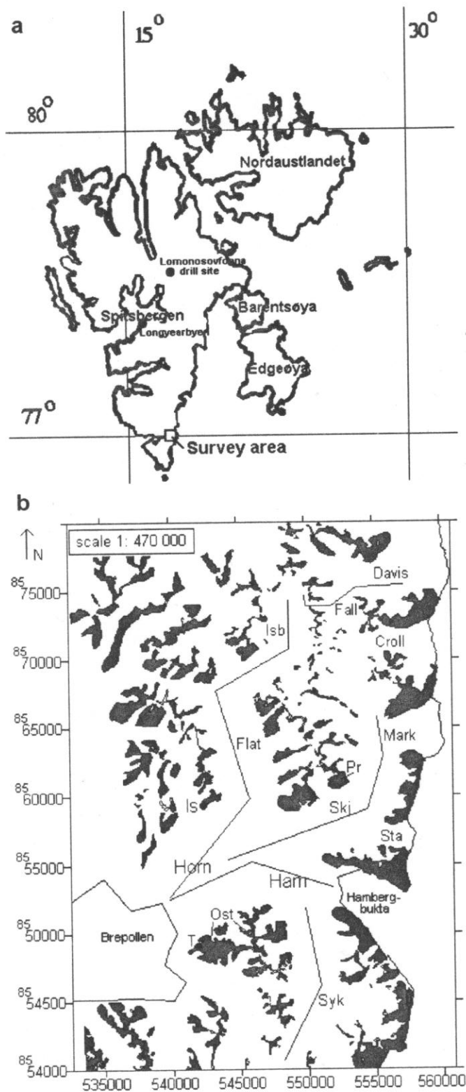
Fig. 1. (a) Location map of Svalbard with the survey area (black outlined rectangle) and the Lomonosofonna drill site (black circle). (b) Detail with place names and surface elevation profiles for Figure 4. Horn, Hornbreen; Ham, Hamborgbreen; Syk, Sykorabreen; Flat, Flatbreen; Isb, Isbroddbreen; Skj, Skjoldfonna; Sta, Staupbreen; Mark, Markhambreen; Croll, Crollbreen; Fall, Fallbergisen; Davis, Davisbreen; Ost, Ostrogradskifjella; Pr, Preikestolen. DGPS base stations at Is (Isingfjellet) and T (Tviryggen) shown by black dots.
