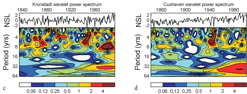
Fig 4. Normalized time series (top plot) and wavelet power spectrum (Morlet) of (a) the NAO winter index and (b) the AO winter index. Normalized sea level time series (NSL) and wavelet power spectrum (Morlet) at Kronstadt (c) and at Cuxhaven (d). Contours are in variance units. In all panels, the black thick line is the 5% significance level using the red noise model; the solid line indicates the cone of influence. The colour bar represents normalized variances.
