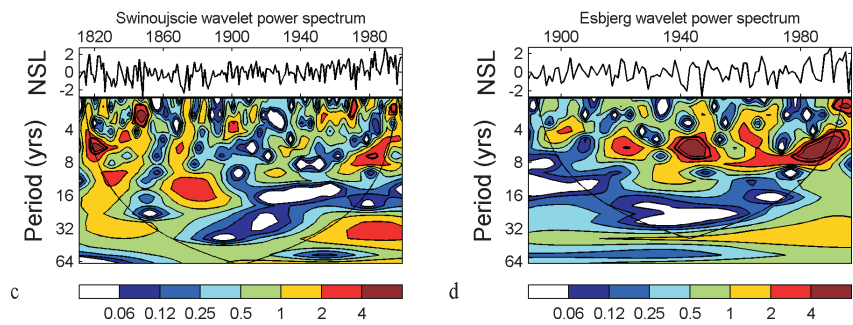
Fig 5. Normalized sea level time series (NSL) and wavelet power spectrum (Morlet) at Brest (a), Aberdeen (b), Swinoujscie (c) and Esbjerg (d). Contours are in variance units. In all panels the black thick line is the 5% significance level using the red noise model; the solid line indicates the cone of influence. The colour bar represents normalized variances.
